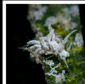
Cuthona sp.3
