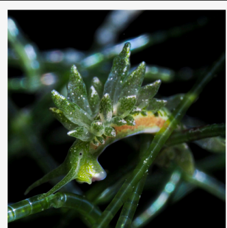
Ercolania viridis
